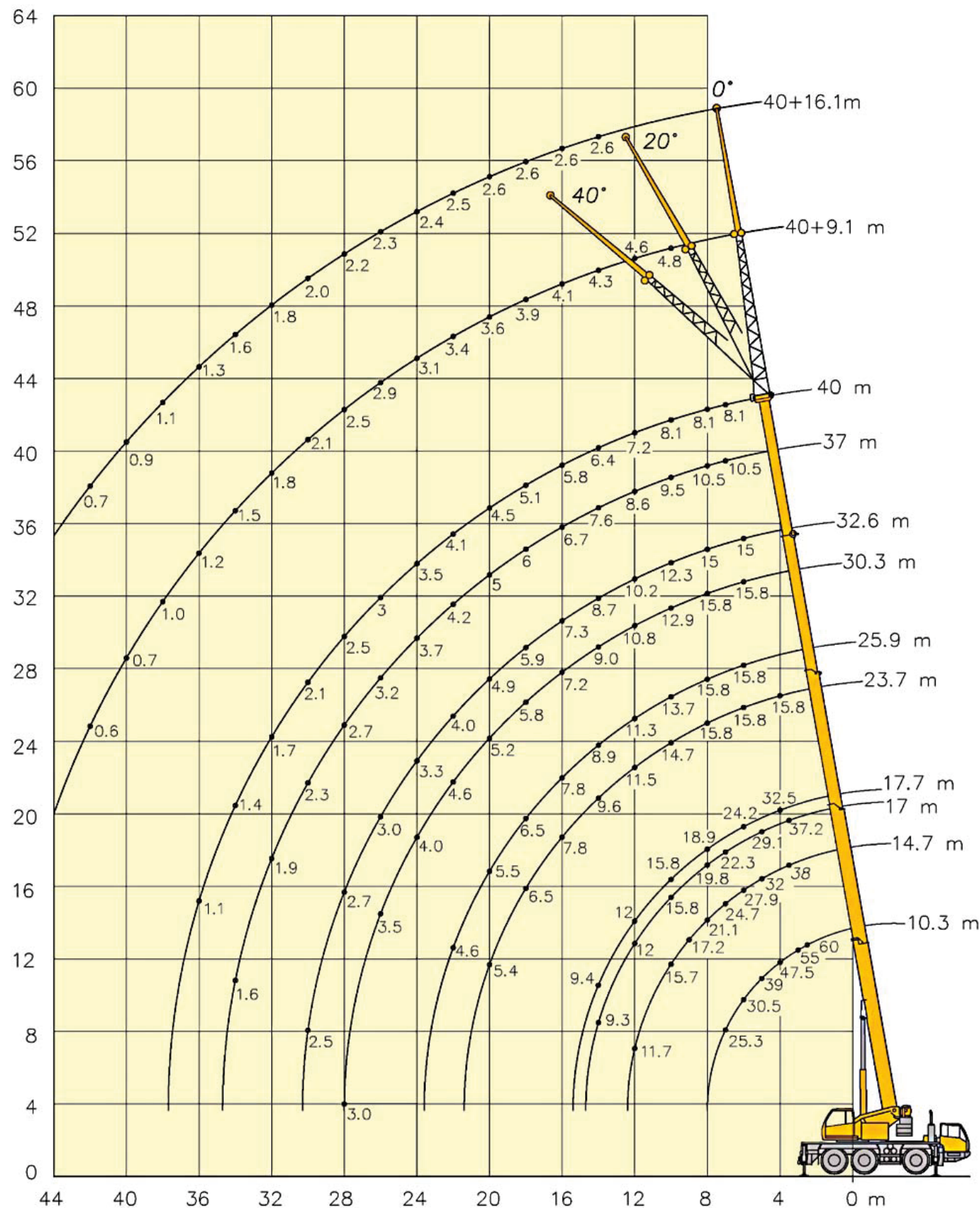
MG 60.3/2
